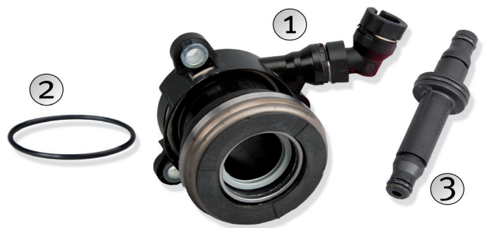
Image 2: LuK CSC 510 0073 10 Current Design
