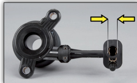
Image 2: LuK CSC 510 0097 10 hydraulic connection 13.3 mm
